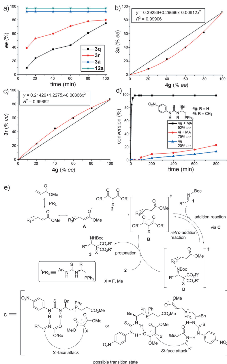
Figure 2. Mechanism study. a) Real-time monitoring of the ee values of the reactions by HPLC analysis using a chiral stationary phase. b,c) Nonlinear effects observed for 3a and 3r. d) Comparison of reaction rates and enantioselectivities of 3a with the catalysts 4g and 4i as determined by ^{19}\text{F} NMR analysis of 3a. The reactions were carried out with 1a (0.12 mmol), 2a (0.10 mmol), and the catalyst (5 mol %) in \text{CH}_2\text{Cl}_2 at room temperature. e) Plausible reaction pathway. MA = methyl acrylate.
